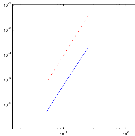
Figure 7: Error measured in the maximum norm for Test 2. The dashed line demonstrates \mathcal{O}(h^4) convergence rate.
